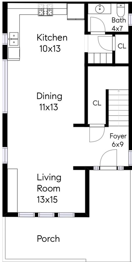
Floor 1
